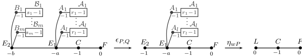
Fig. 2.1. The morphisms (Y, B) \xrightarrow{\epsilon_{P,Q}} (W, B) \xrightarrow{\eta_{wP}} (\mathbb{F}_1, F \triangleright C \triangleright L) when P(0) \neq 0 . A block with label t consists of a zigzag of t (-2) -curves.
