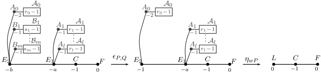
Fig. 2.2. The morphisms (Y, B) \xrightarrow{\epsilon_{P,Q}} (W, B) \xrightarrow{\eta_{wP}} (\mathbb{F}_1, F \triangleright C \triangleright L) when P(0) = 0 and Q(0) \neq 0 .
