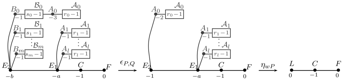
Fig. 2.3. The morphisms (Y, B) \xrightarrow{\epsilon_{P,Q}} (W, B) \xrightarrow{\eta_{wP}} (\mathbb{F}_1, F \triangleright C \triangleright L) when P(0) = Q(0) = 0 .
